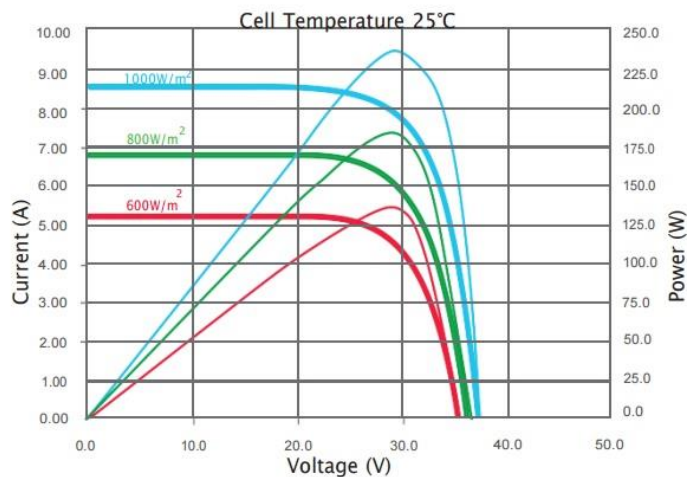
Current, Power vs. Voltage Characteristics of ASW-240P
